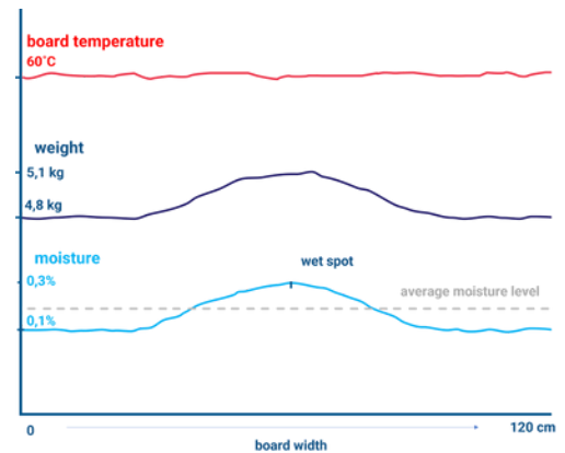
Profiling of single plasterboards
